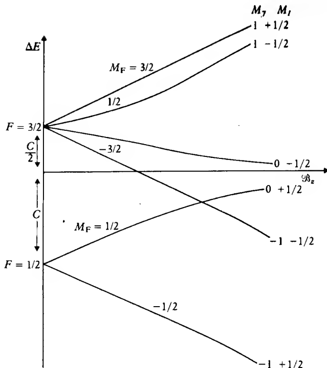
8.6 Behaviour of the hyperfine splitting as a function of \mathcal{B}_z for I = 1/2 , J = 1 (arbitrary scale). In the weak field case to the left of the diagram the states are classified by F, I, J, M_F and in the strong field case to the right by I, J, M_J and M_I , (see equations [8.49] and [8.53] respectively). To connect the strong and weak field limits we must remember that M_F = M_I + M_J , always and levels with the same M_F or M_J never intersect each other. If the field strength increases even further, then the spin-orbit coupling breaks down and the states are classified by L, S, I, M_L, M_S (this is the extreme Paschen-Back effect).
